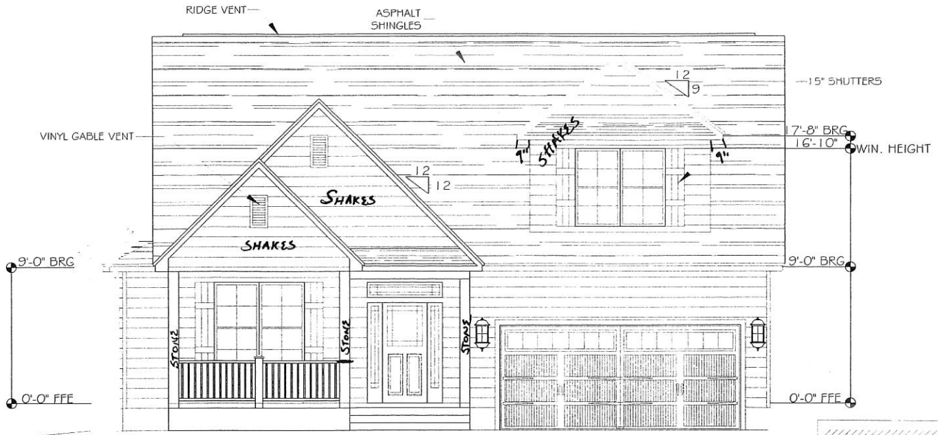
FRONT ELEVATION
